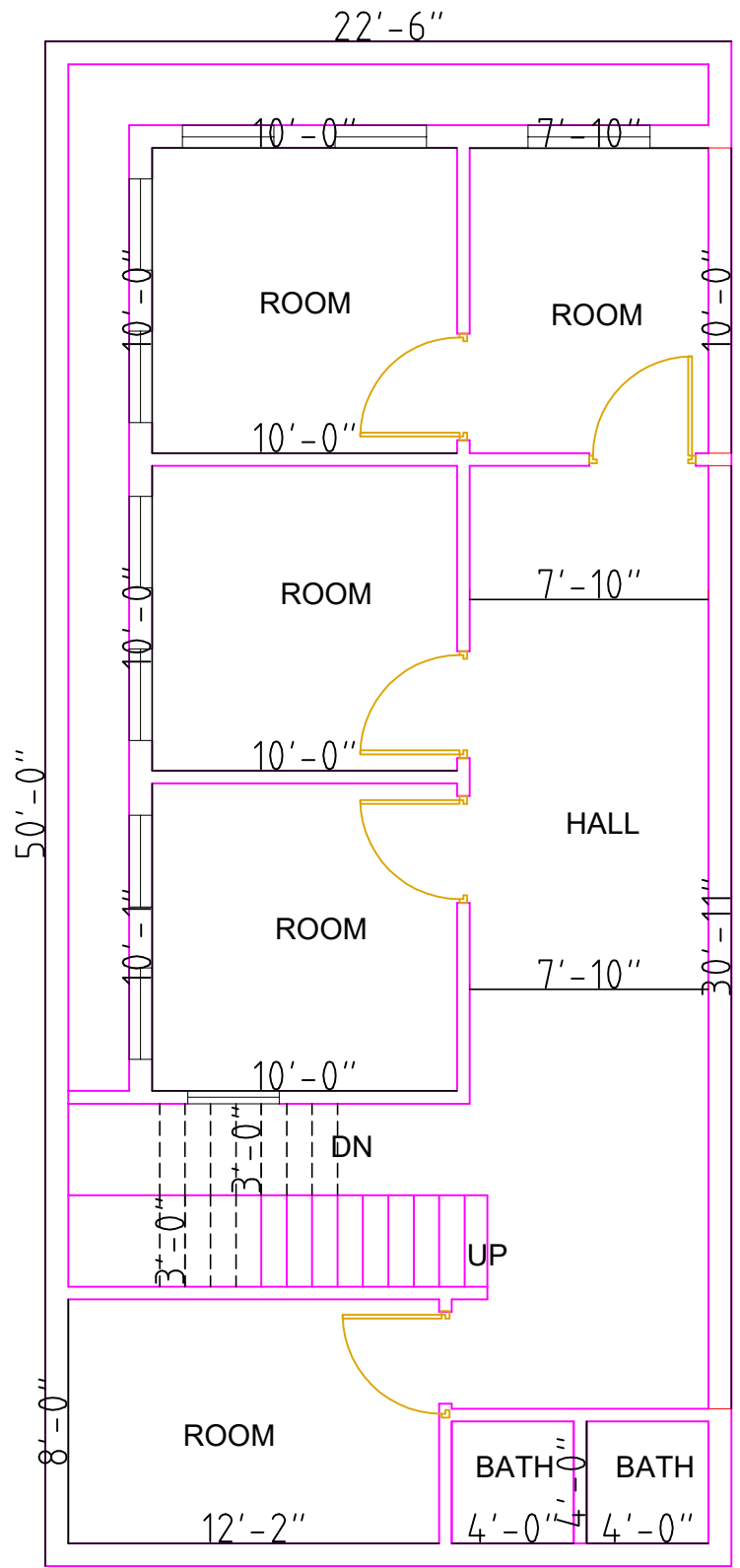
FIRST FLOOR PI AN
