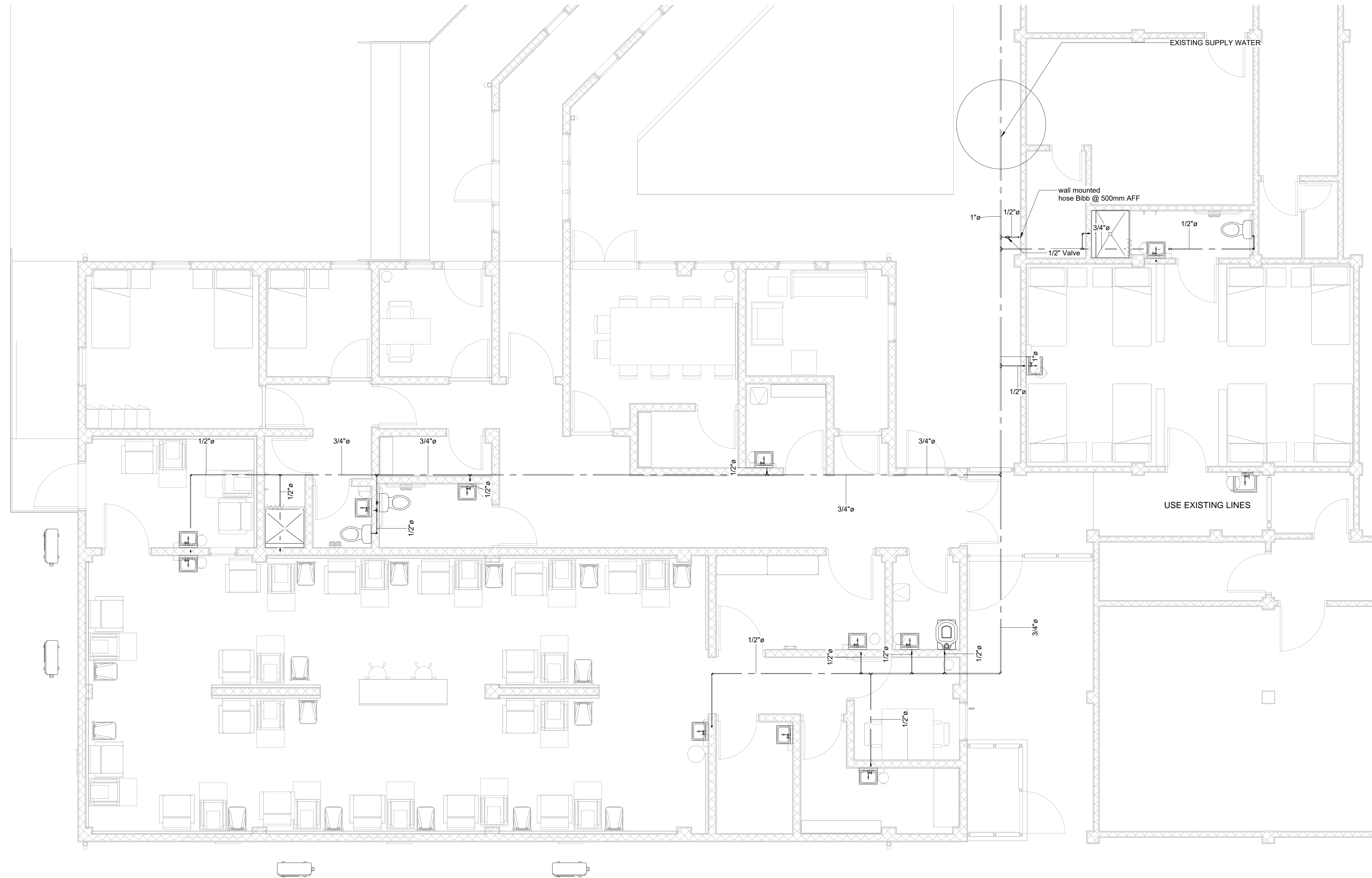
Plumbing Plan - DOMESTIC COLD WATER
