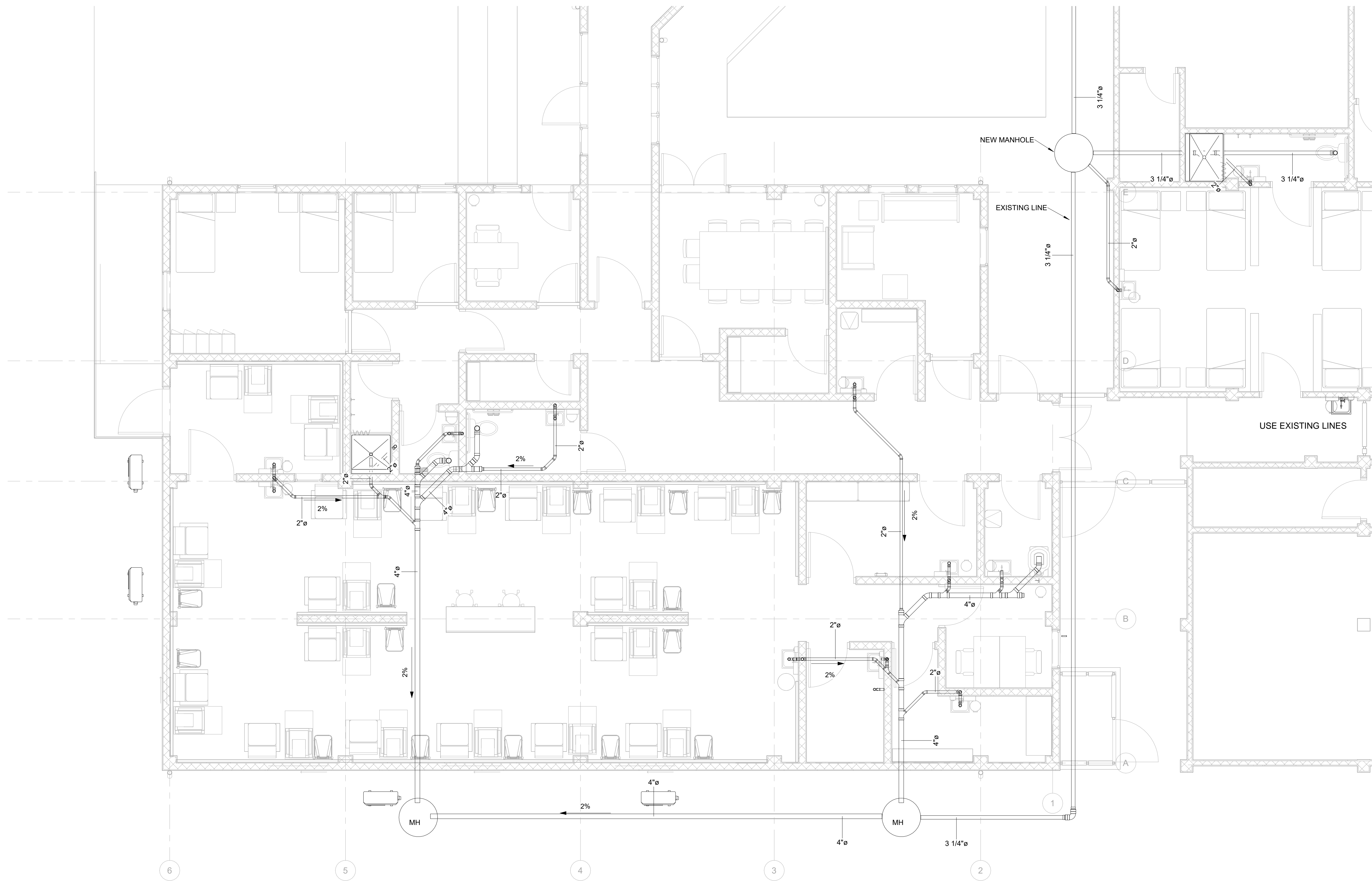
1 Plumbing Plan - SANITARY LEVEL 1 SCALE 1/4" = 1'-0"
