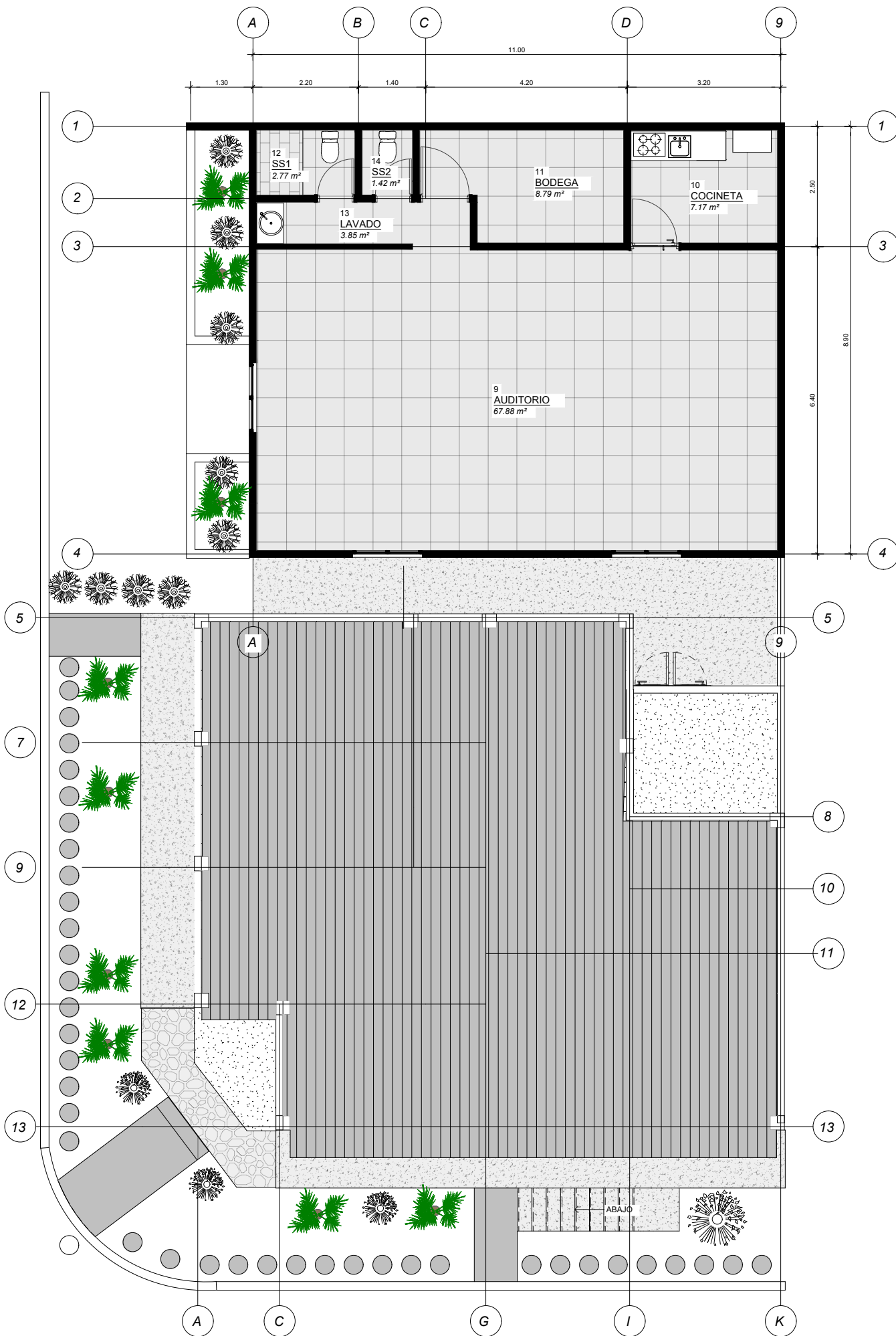
1 PLANIMETRIA GENERAL 1:75
