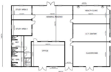
PLAN VIEW - KOTOBABI NO. 2 CLUSTER OF SCHOOLS LIBRARY 65 X 40 FT
