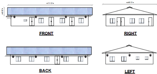
ELEVATIONS - KOTOBABI NO. 2 CLUSTER OF SCHOOLS LIBRARY 65 X 40 FT
